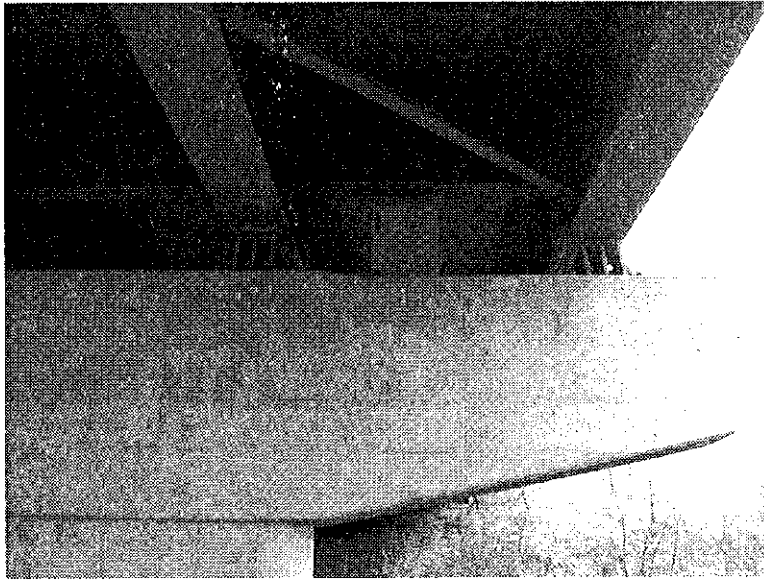
Figure 53. Photograph of DAS enclosure on Pier 2.
