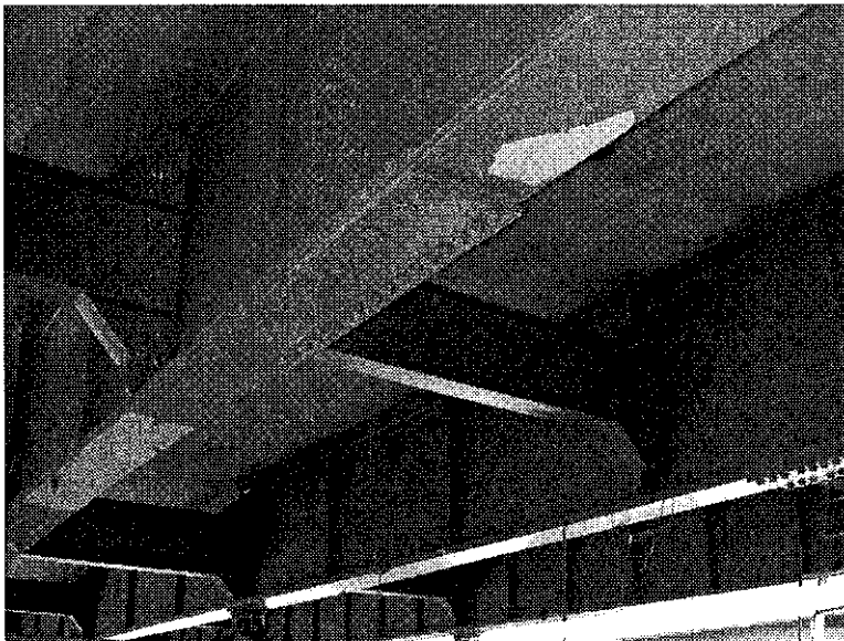
Figure 5. Photograph of underside of the bridge looking northwest.
