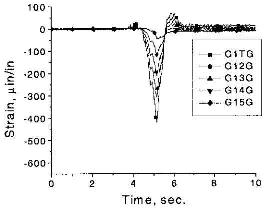
c. Middle row bolts tight.
