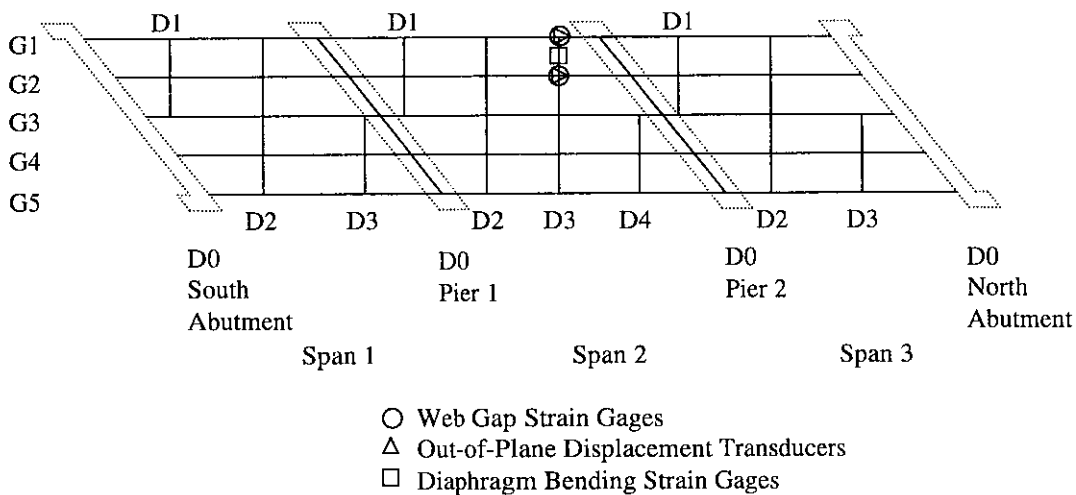
Figure 34. Plan view of gage placement.
